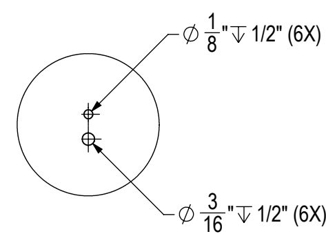
OVERLAY CLIP MTG HOLES DETAIL A SCALE 1 : 2
