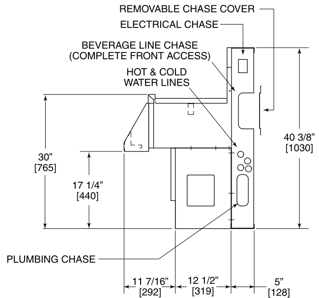
PEDESTAL BASE END VIEW
