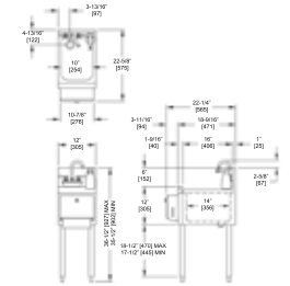
End View Hand Sink
