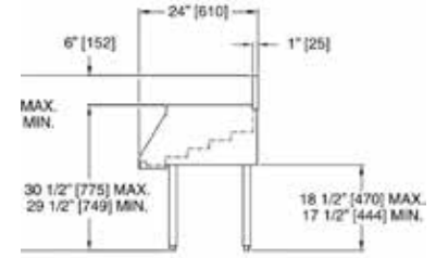
End View Liquor Display
