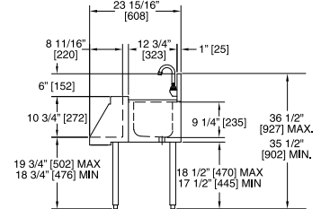
End View Blender Station w/Sink
