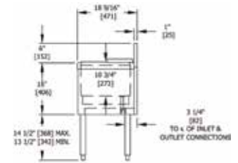
End View Standard Ice Chest
