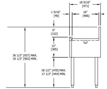
End View Drainboard
