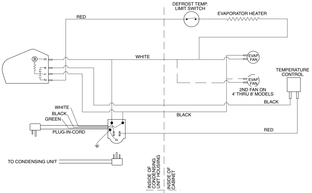
WIRING DIAGRAM FOR LOW TEMPERATURE BOTTLE COOLER – BC48LT, BC60LT & BC72LT
